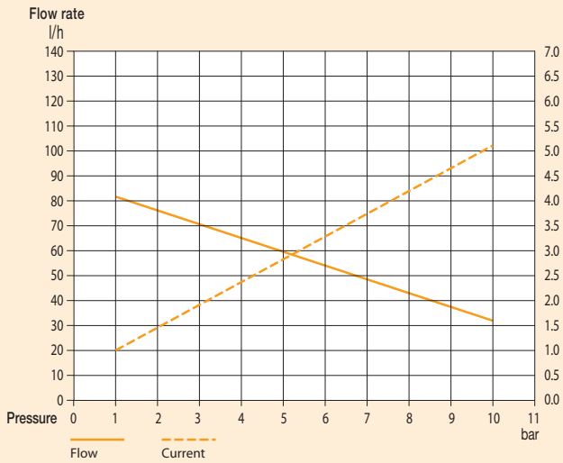
GA0072 - 24 V 42x100 mm BRUSHLESS MOTOR (90-93-02)
