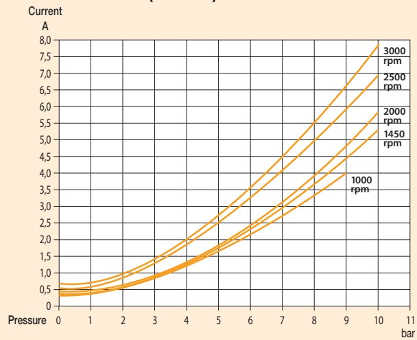
GA0102 - 24 V 42x100 mm BRUSHLESS MOTOR (90-93-02)
