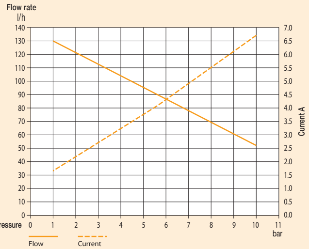
GA0072 - 24 V 42x100 mm BRUSHLESS MOTOR (90-93-02)
