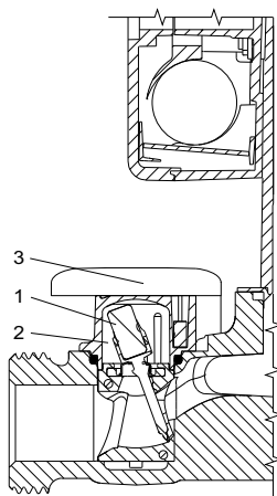
Fig. 9 Flow switch of UPA 15-120
