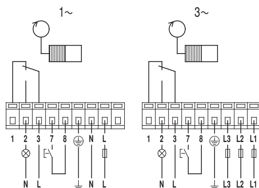
Fig. 36 Operating indication
