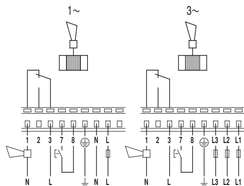
Fig. 37 Fault indication
