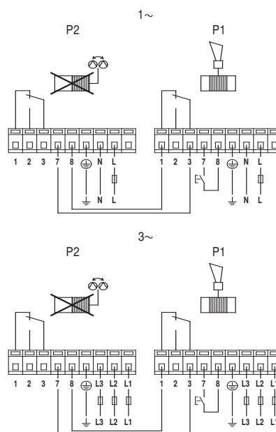
Fig. 39 Standby operation
