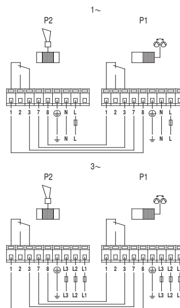
Fig. 38 Alternating operation
