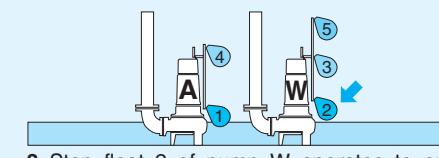
3 Stop float 2 of pump W operates to end water discharge. At this time, alternation start float 3 of pump W rests for one discharge operation.
