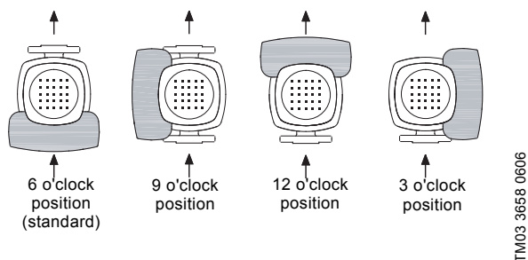
Fig. 5 Terminal box positions
