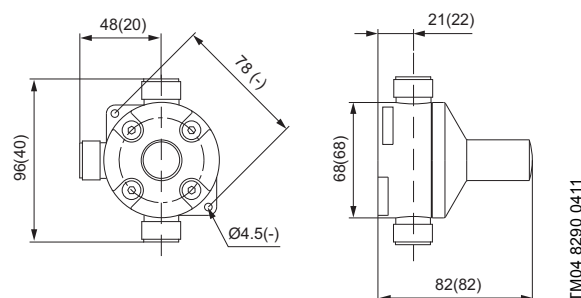
Fig. 44 Pressure relief valve. Dimensions in brackets apply to stainless-steel version.
