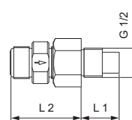
Fig. 37 Standard injection unit, stainless-steel version
