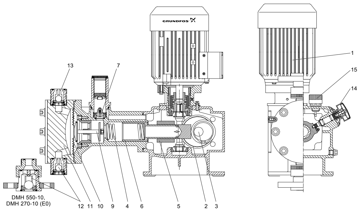
Fig. 22 Sectional drawing, DMH model 255
