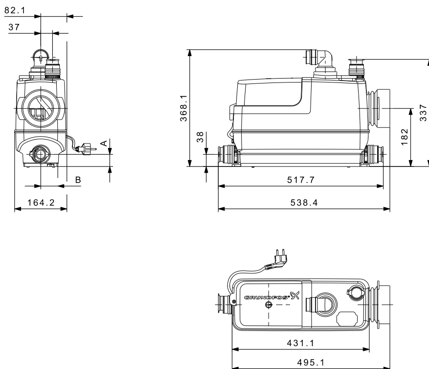
Fig. 27 Dimensional drawings, Sololift2 CWC-3
