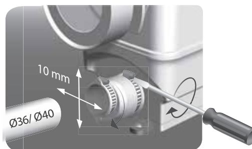
Fig. 35 Height and side alignment possible when using Ø36/40 inlet pipes
