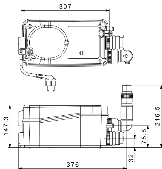
Fig. 44 Dimensional drawings, Sololift2 D-2
