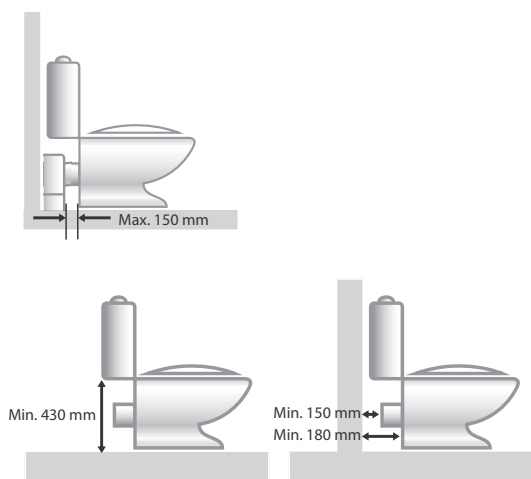
Fig. 15 Distances to be observed
