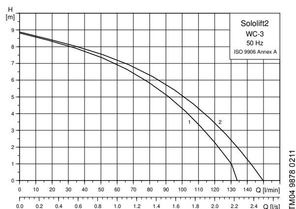
Fig. 18 Performance curves, Sololift2 WC-3
