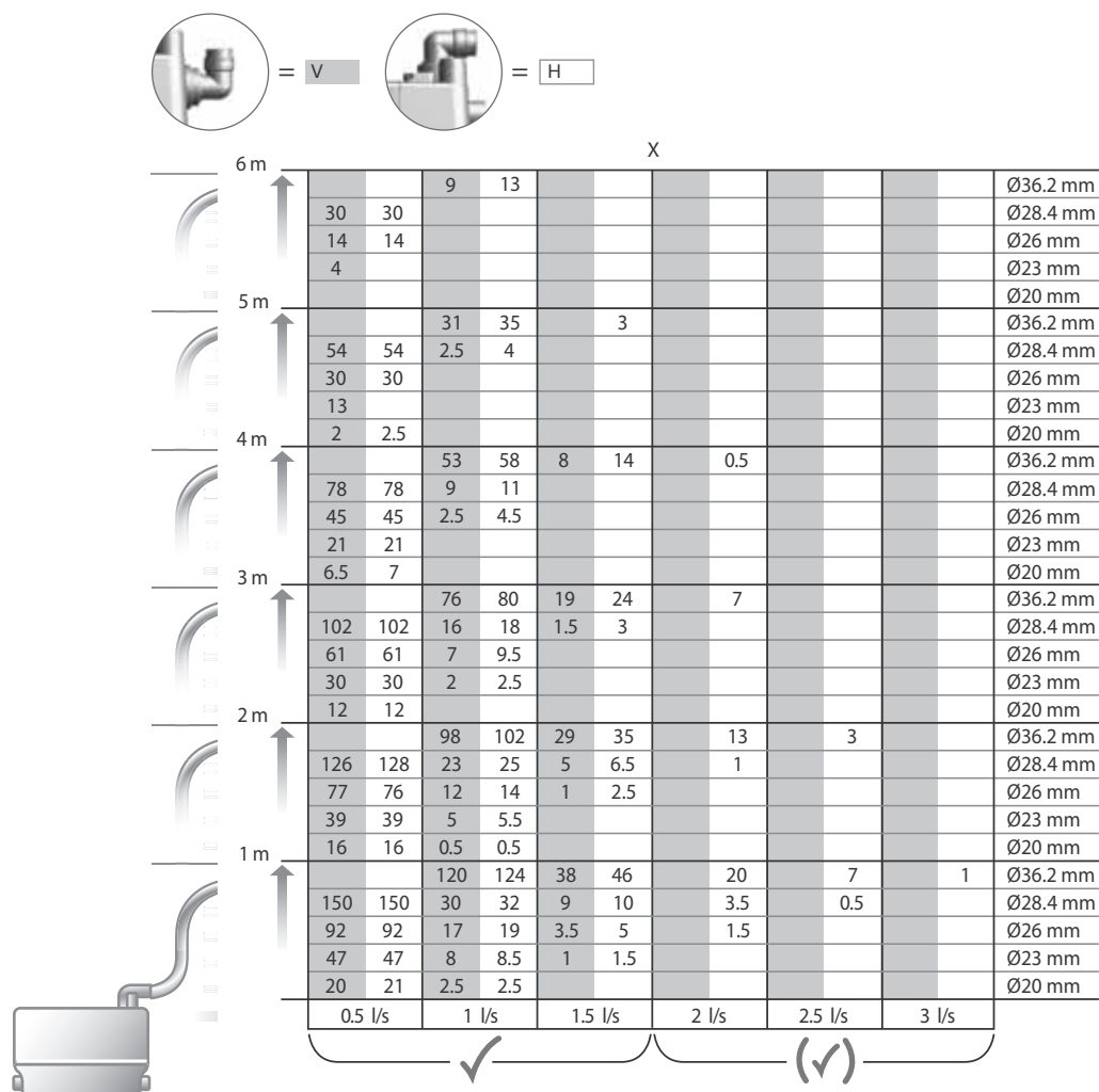
Fig. 30 Pipe length and height in relation to inner pipe diameter and required discharge capacity
