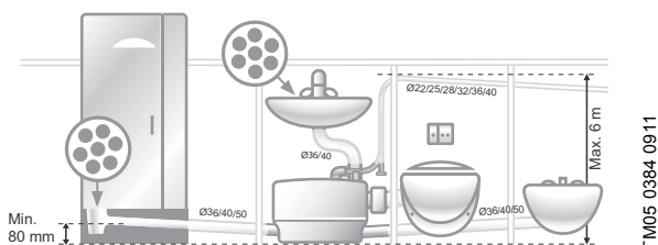
Fig. 23 Example of installation
