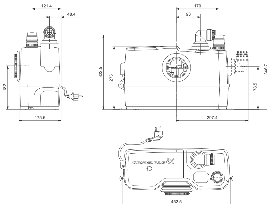
Fig. 10 Dimensional drawings, Sololift2 WC-1
