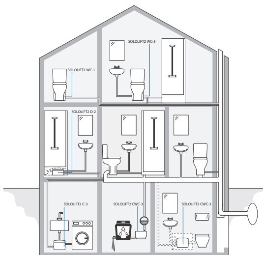
Fig. 1 Examples of application
