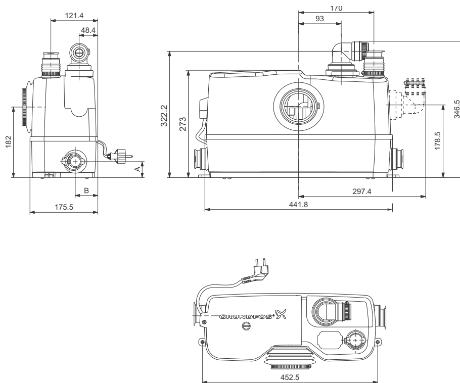
Fig. 19 Dimensional drawings, Sololift2 WC-3
