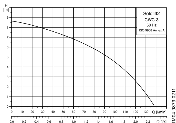
Fig. 26 Performance curves, Sololift2 CWC-3
