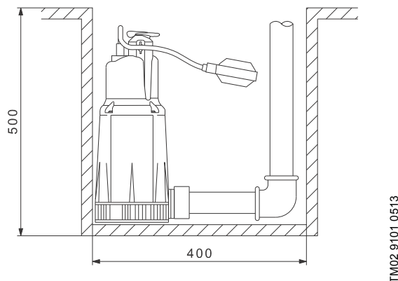
Fig. 23 Minimum dimension for the pit for KPC 600 A with automatic float switch
