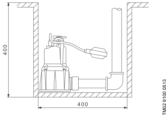
Fig. 22 Minimum dimension for the pit for KPC 300 A with automatic float switch
