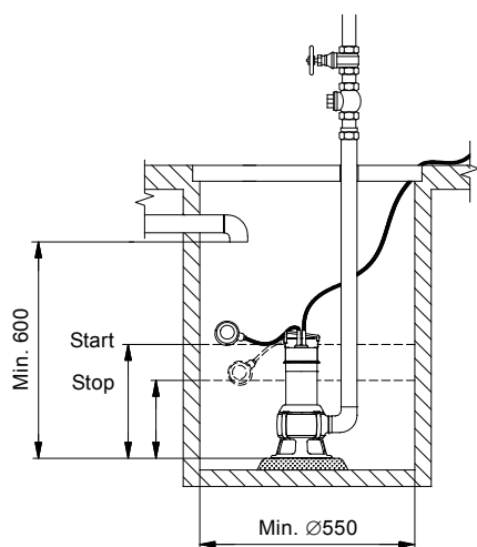
Fig. 49 Minimum well dimensions, Unilift AP50B
